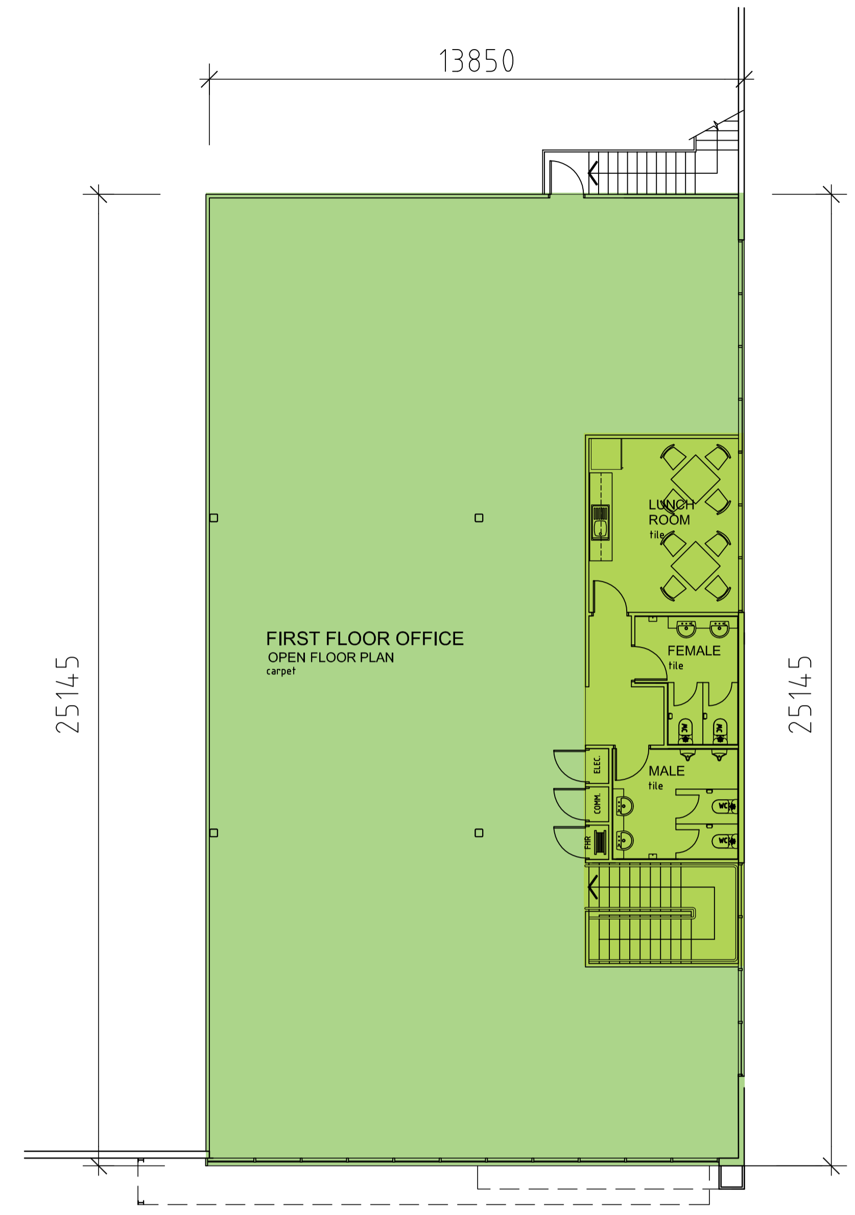
FIRST FLOOR PLAN AREA = 340 SQM
